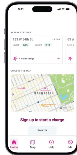
Driver App
